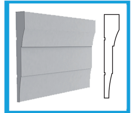
KS 15 90 x 9 cm
