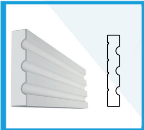
S11 20 x 4 cm
