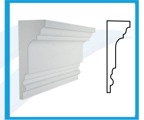
KS 6 30 x 12 cm
